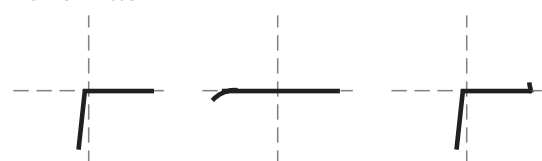
Typ: Normale Diode Pole: Kathode-Anode Anschlüsse: (CT-Masse)
